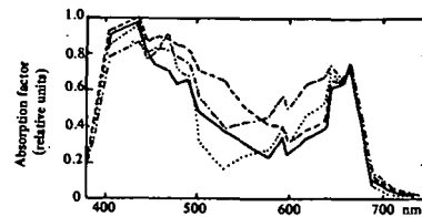
Figure 5-1 In vitro absorption of the chlorophyllian pigments of four ornamental plants (Dodillet, 1961)
