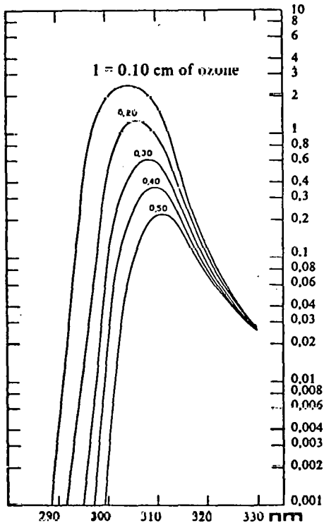
Figure 5-3 Distribution of the specific erythemal spectral irradiance of the global solar radiation on a horizontal surface (altitude: sea level; sun elevation; 45^\circ ; very bright, clear sky) (Dogniaux, 1954)
