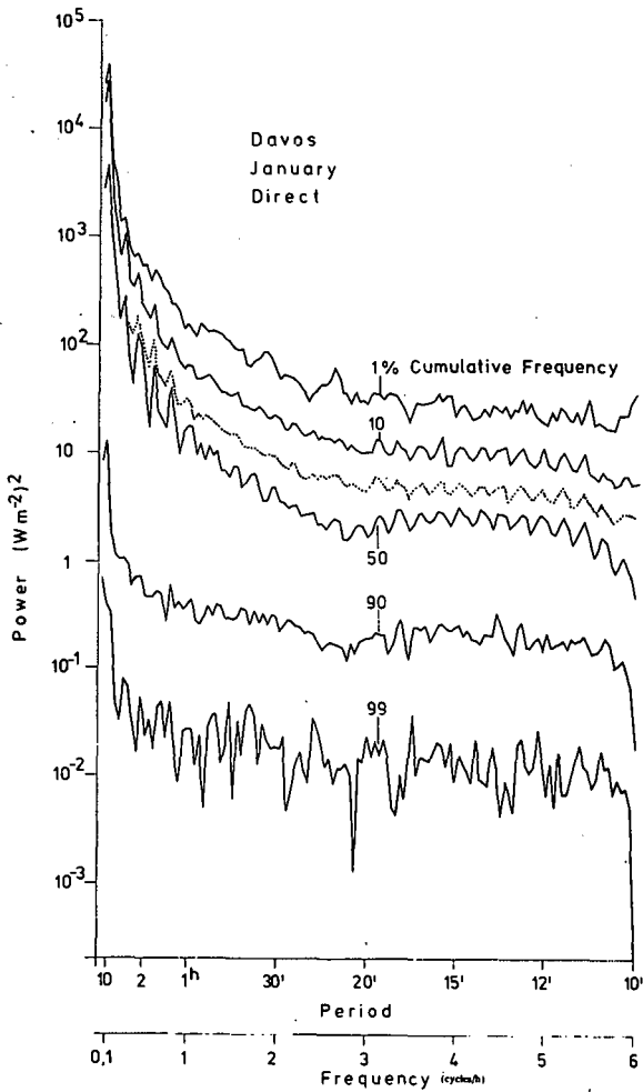
Figure 8-23 Same as Figure 8-22 except for direct radiation recorded on a horizontal surface during 390 January days at Davos.
