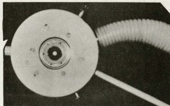
Figure 6-10 A Fritschen type net pyrradiometer
