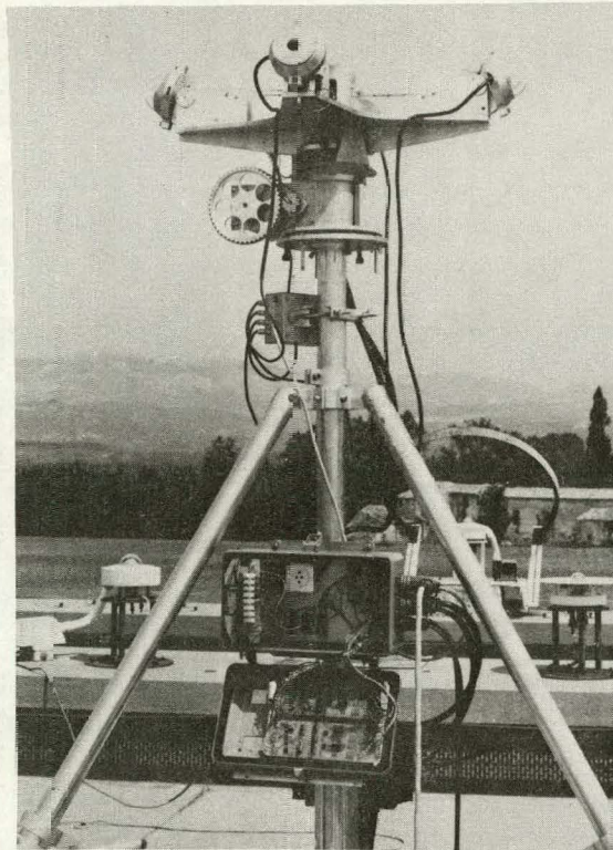
Figure 8-30 Main components of the mobile system for solar radiation measurements
