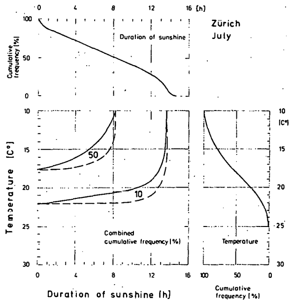
Figure 8-41 Comparison of bivariate cumulative frequency curves with those obtained by simply multiplying the corresponding univariate frequencies.
