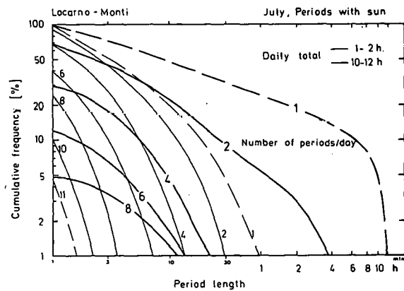
Figure 8-15 Cumulative frequency distribution of the number of sunny periods per day for July, Locarno-Monti. Thin curves were drawn for days having 1-2 h of daily sunshine; and thick curves, for 10-12 h of daily sunshine.
