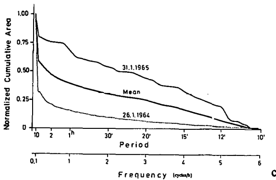
8-20-c Normalized cumulative area for the clear-day (lower curve) and the overcast day (upper curve) together with the mean over 280 January days.
