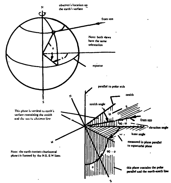
Figure 2-9 Geocentric and observer-centric views showing pertinent angles involved. Note: north, south, east, west lines are tangent to the earth's surface.
