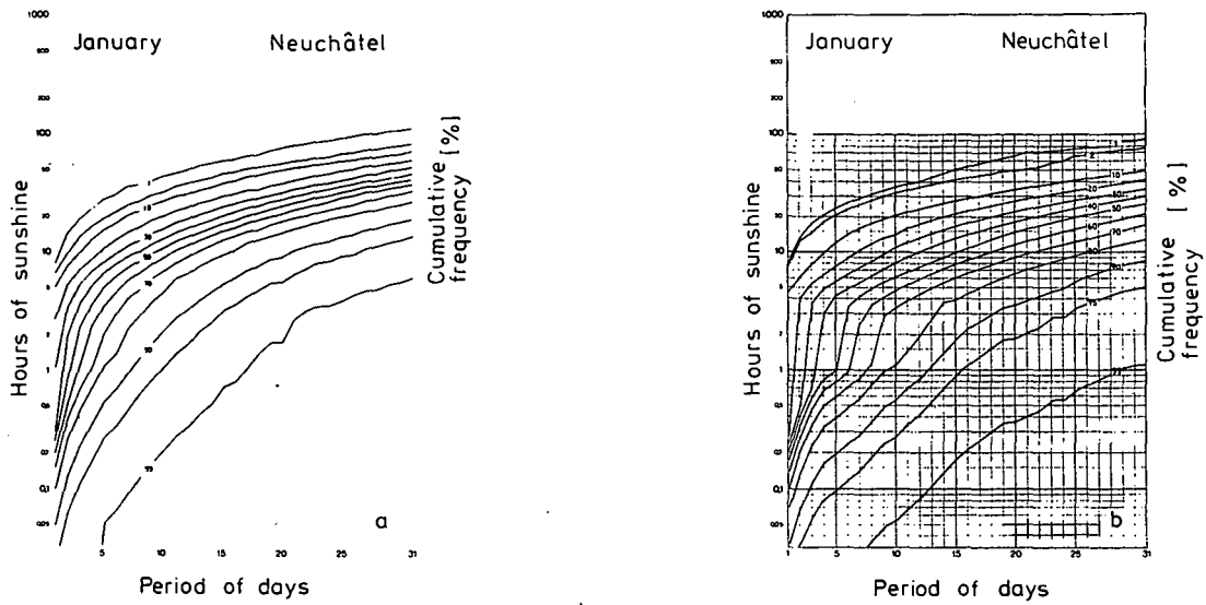
Figure 8-7 Cumulative frequency distribution of sunshine hours accumulated over periods of n \leq 31 consecutive days in January for Neuchâtel. The entire 40-year (1931-1970) period of record was used: a) to its full extent. Example: There is a chance of about 5% of receiving 25 h of sunshine during a 10-day period, but it is almost certain (99% frequency curve) that at least 10 min of sunshine would be received. b) restricted to days with at least one uninterrupted period of sunshine lasting at least 2 h.
