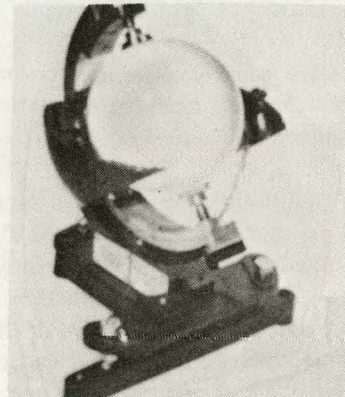
Figure 9-1 The Campbell-Stokes sunshine recorder
