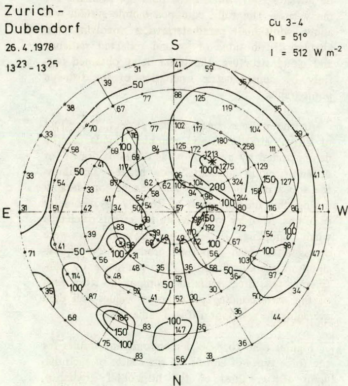
Figure 8-35 Same as Figure 8-31, except for a cloudy sky covered by 3/10 - 4/10 of cumulus cloud and for a solar height of 51°.
