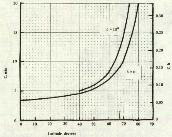
Figure 2-12 Sunrise-sunset time correction, C
