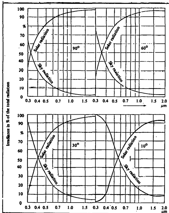
Figure 5-9 Percentage of solar radiation and sky radiation at different altitudes of the sun (cloudless days).
