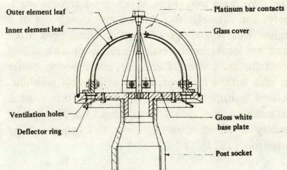
Figure 9-2 Cross-section of sunshine sensing element (Sumner, 1966)
