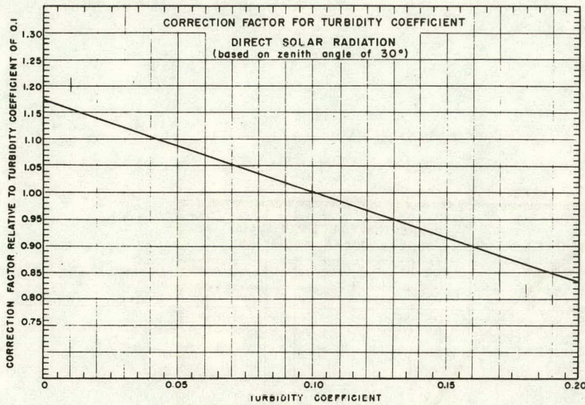
Figure 8 Graph for determination of direct radiation correction factor for turbidity. For example, if the turbidity coefficient is 0.15 then the correction factor for turbidity is 0.92.
