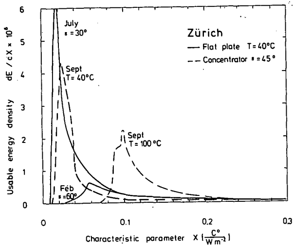
Figure 8-42 Monthly distributions of the usable energy density as a function of the weather-dependent characteristic parameter
