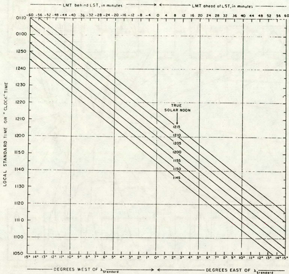
Figure 1 Determination of Local Standard Time from True Solar Noon, TSN, and degrees of longitude east or west of standard latitude, \lambda_{standard} . For example, suppose a calculation is desired at the Greensboro, North Carolina, U. S. A. airport ( 79^{\circ} 57' W ) on March 28. The clock time is Eastern Standard Time and the standard meridian, \lambda_{standard} , is 75^{\circ} W (Table 9). Greensboro is therefore almost 5^{\circ} west of the standard meridian: 79^{\circ} 57' - 75^{\circ} = 4^{\circ} 57' . On March 28, the TSN is 1205 from Table 2. Entering 1205 for True Solar Noon along the sloping lines and the longitudinal difference of just under 5^{\circ} (west) as the horizontal axis. The corresponding Local Standard or "clock" Time is 1225. At 1225 local time at Greensboro airport the sun will be most direct overhead on March 28. Note that 5^{\circ} difference is 20 minutes later at Greensboro than for a location on the 75th meridian (see top of figure and check: 1225 - 1205 = 20 min.). LMT stands for Local Mean Time, or the Local Standard Time at the 75th meridian. It takes 20 minutes for the sun to traverse the almost 5^{\circ} of longitude between the 75th meridian and the approximately 80th meridian.
