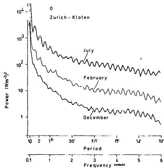
Figure 8-25 Same as Figure 8-24 except global radiation recorded on a horizontal surface at Zurich-Kloten during December (273 days), February (232 days) and July (300 days).
