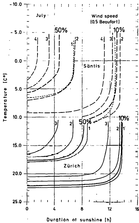
Figure 8-40 Same as Figure 8-39, except including wind speed as a third variate. Curves are drawn only for the 10 to 50% cumulative frequency levels.
