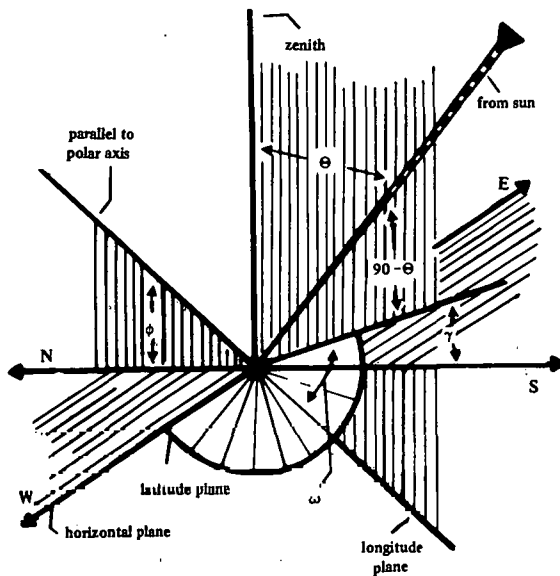
Figure 2-10 Observer-centered view with zenith vertical and north-south/east-west plane horizontal. Note: latitude, \phi , in vertical plane containing N-S axis. Hour angle, \omega , in latitude plane is angle between the N-S zenith plane and plane containing the elevation angle, 90 - \Theta , which is a vertical plane containing the sun line. Zenith angle, \Theta , is in the same plane as 90 - \Theta . Azimuthal angle, \gamma , is in the horizontal plane and gives the angle in this plane between the N-S; i.e., observer longitude plane and the plane containing the zenith and the sun line.
