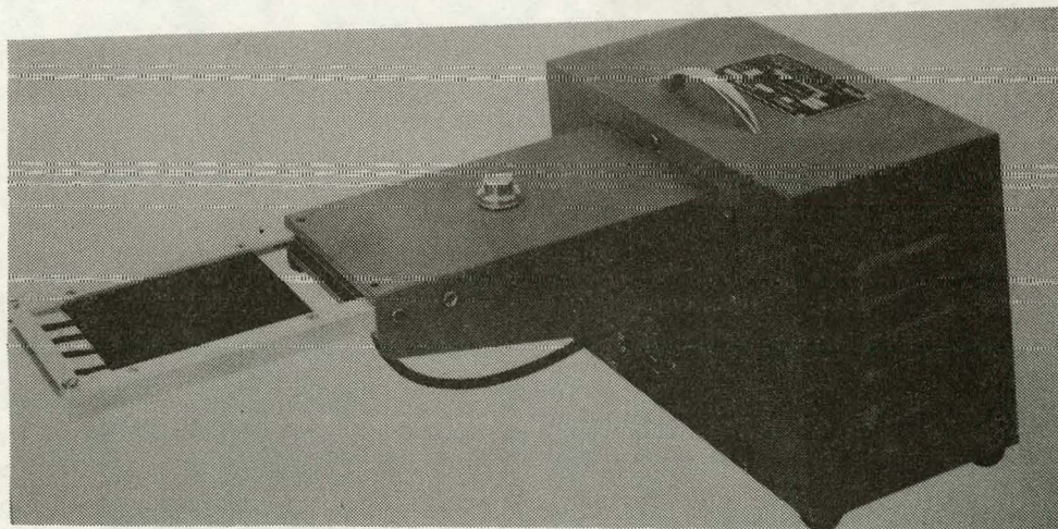
Figure 6-6 An unshielded net pyrriometer of the Gier and Dunkle design. Manufactured by Teledyne Geotech.
