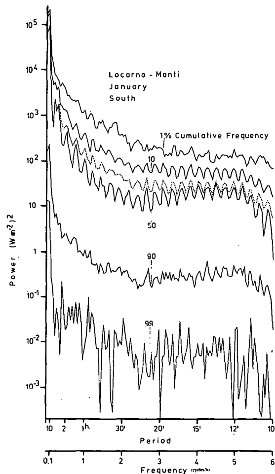
Figure 8-22 Cumulative frequency distribution of statistical power spectra of global radiation falling on a south-facing vertical surface on January days at Locarno-Monti. The dotted curve marks the mean statistical spectrum. The ordinate is enlarged 2:1 compared with Figure 8-20.
