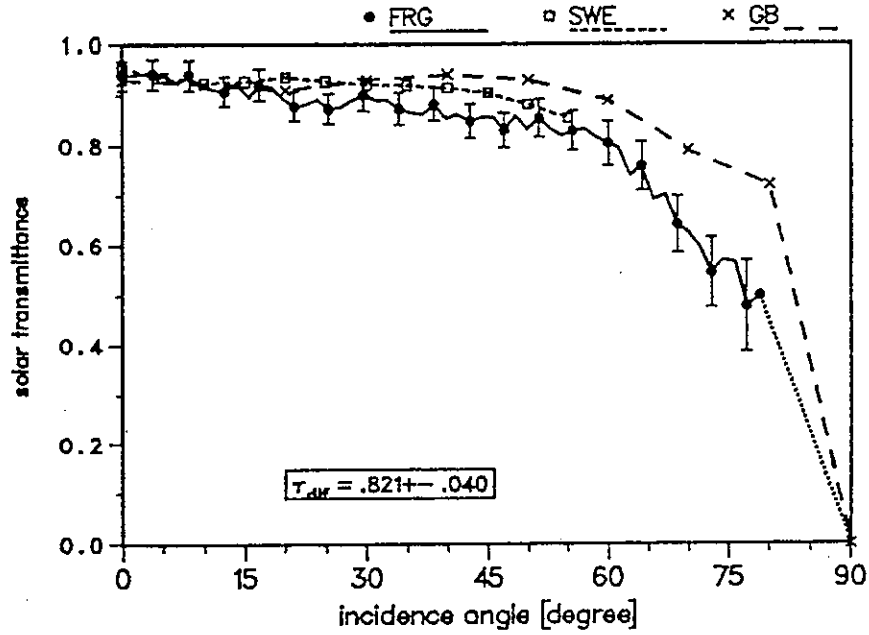
Fig. 8. Solar transmittance T_S(A) verses incidence angle for a 5 cm Arel polycarbonate honeycomb sheet.
