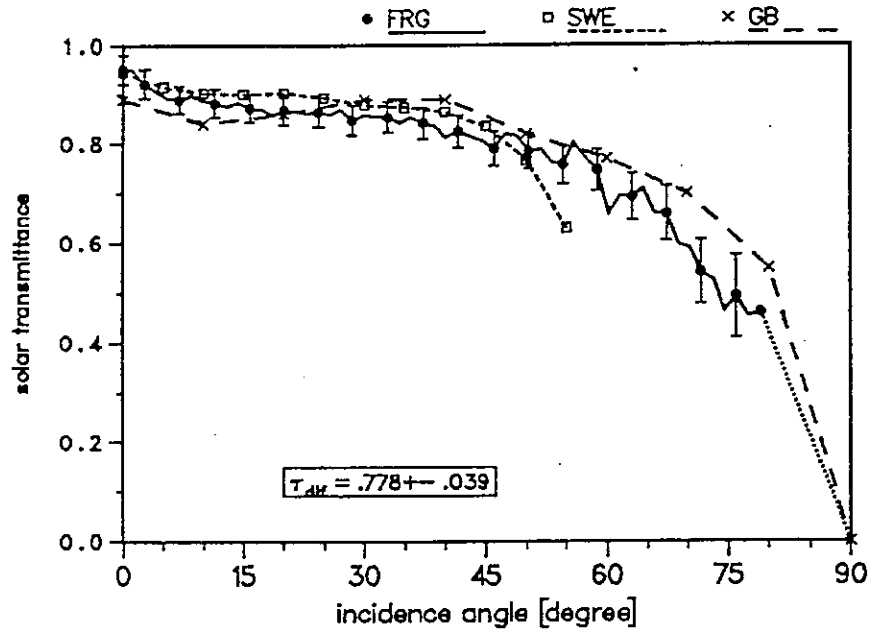
Fig. 9 Solar transmittance T_S(A) verses incidence angle for a 10 cm Arel polycarbonate honeycomb sheet (sample A).
