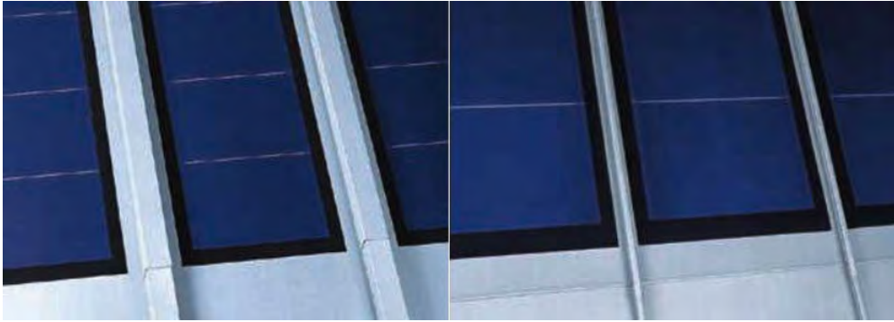
Fig. 3.B.43: solar laminate integrated into metal roof system Left: Click roll cap jointing, Right: Standing seam jointing, © Rheinzink
