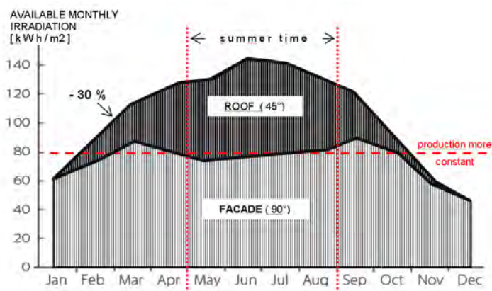
Fig. 4.12: Comparison of the monthly sun radiation available on a 45° south oriented tilted surface vs. a vertical south oriented surface in Graz, Austria (47° latitude). Data from W.Weiss, I.Bergmann, AEE-Intec.
