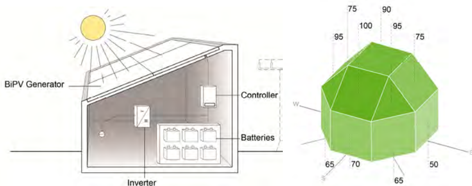
Fig. 3.B.9: Left – Stand alone system scheme. Right - Annual irradiation vs. orientation. (© SUPSI, ISAAC)
