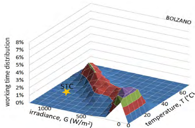
Figure 3.B.11: Working time distribution of a PV plant in Bolzano (Northern Italy) monitored for one year [3-B.2]. STC are rarely met.
