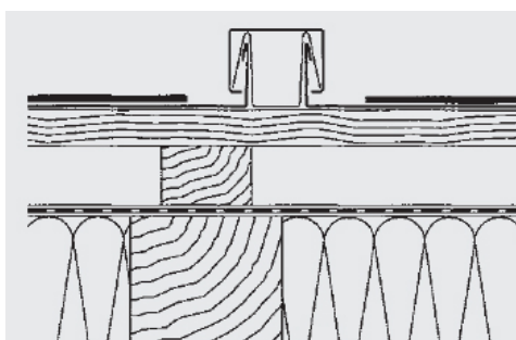
Solar PV Click Roll Cap System, © RheinZink
