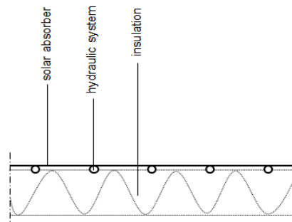
Fig 3.A.6 a- b: Unglazed flat plate collectors as roof covering (left). Right: typical unglazed flat plate collector's cross section and main composition elements.
