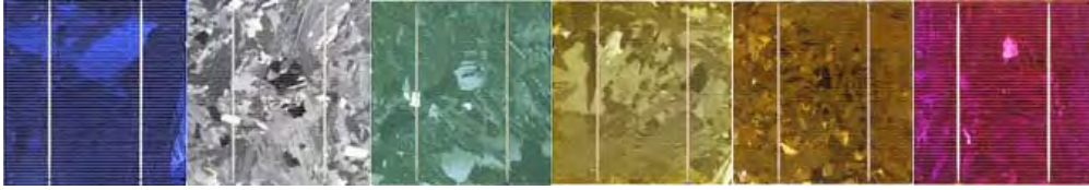
Fig. 3.B.35. multocrystalline silicon wafers; first the blue antireflective standard colour with the best efficiency, the second is the original wafer without reflective layer, then cells with other colours that have different anti-reflective layers, © Sunways
